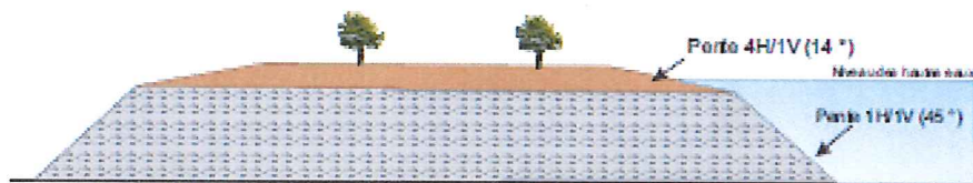
(E) Triple berge
